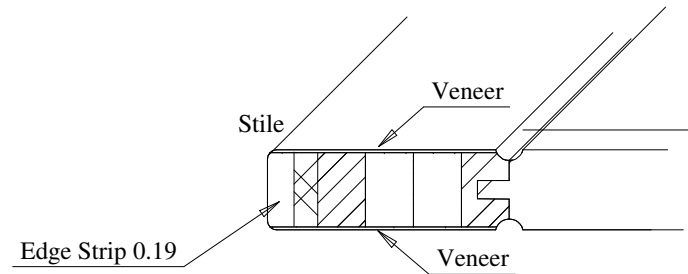
Panel Profile
