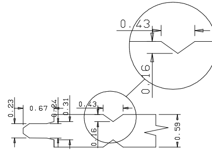
Panel Profile
