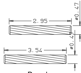
Dowel
